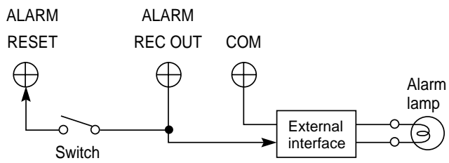
[ALARM REC OUT] alarm recording mode signal output terminal
